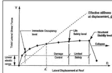
Figure 1. Building Collapse Level
