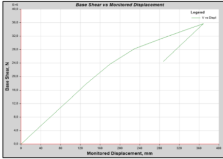
Figure 11. The capacity curve of 4-story soft soil OMRSF
