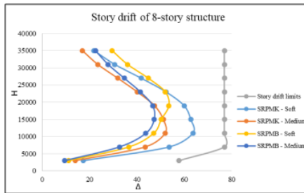
Figure 7. Graph Story drift of 8-story
