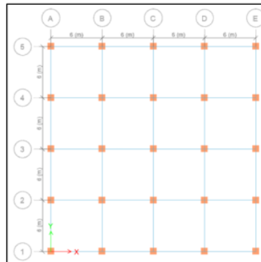
Figure 2. The layout of structure planning
