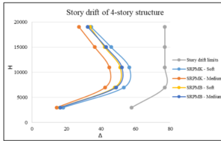
Figure 6. Graph Story drift of 4-story
