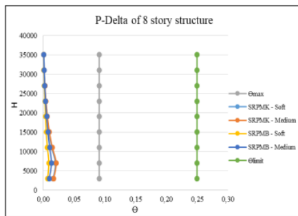
Figure 9. Graph P-Delta of 8-story
