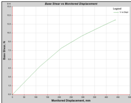
Figure 12. The capacity curve of 8-story soft soil SMRSF
