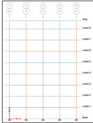
Figure 4. Side view of the 8-story structure
