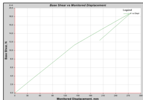
Figure 10. The capacity curve of 4-story soft soil SMRSF
