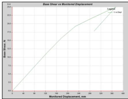
Figure 13. The capacity curve of 8-story soft soil OMRSF
