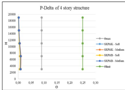
Figure 8. Graph P-Delta of 4-story
